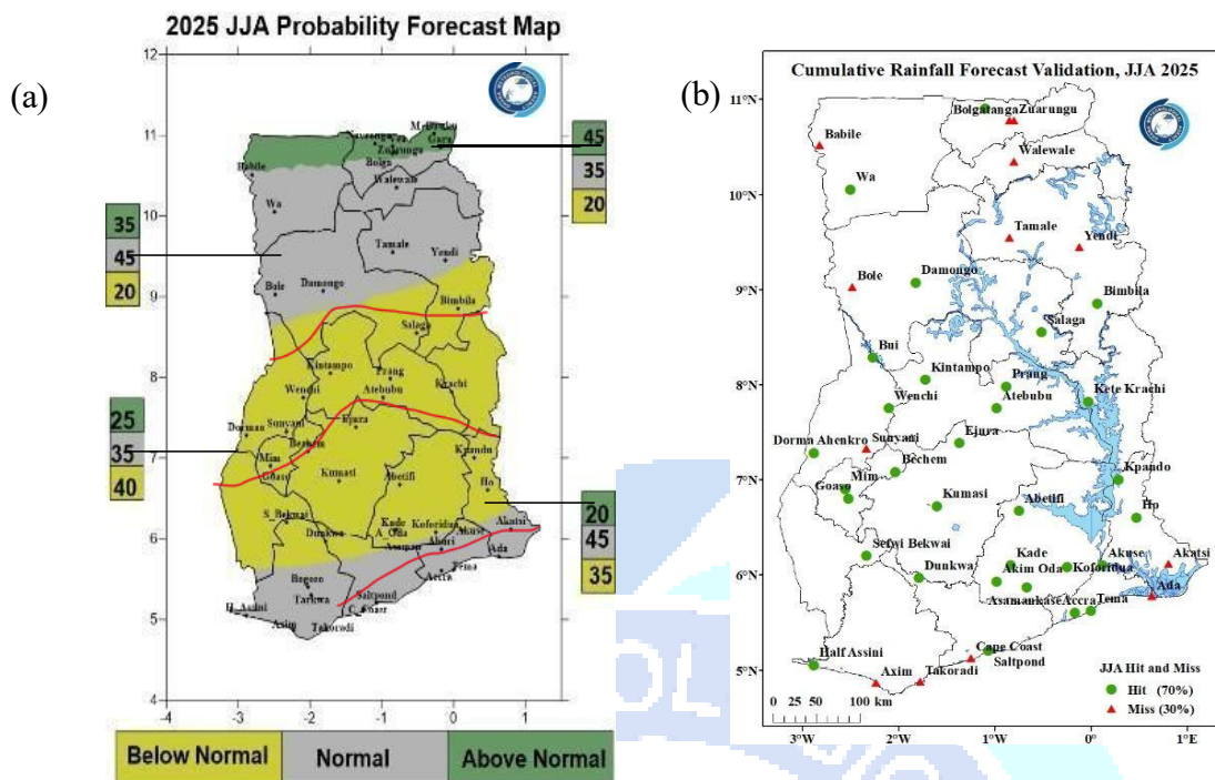
Figure 4: (a) JJA Probability Forecast 2025 (b) Verification Map 2025
