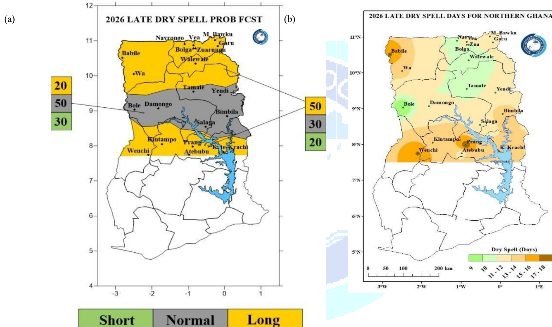
Figure 14: (a) Late Dry Spell Probability Map 2026 (b) Late Dry Spell Forecast Map 2026
