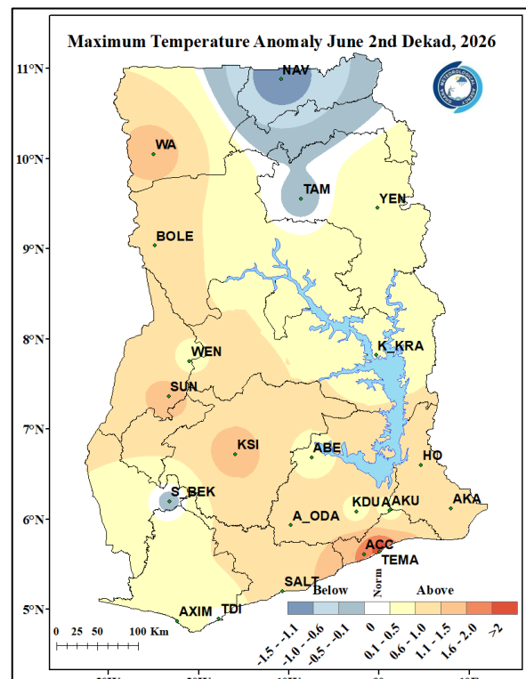
Figure 5b. Max. Temperature Anomaly June 2nd Dekad, 2026
