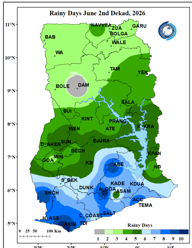
Figure 3b. Rainy Days June 2nd Dekad, 2026
