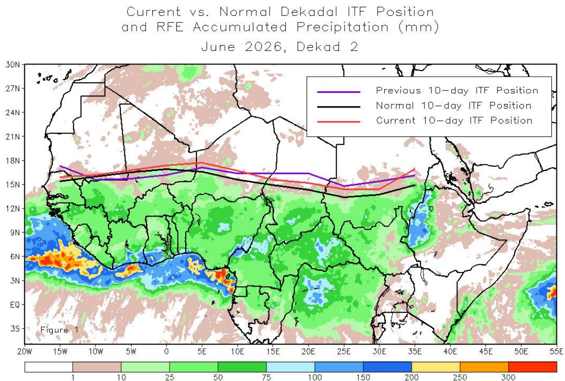
Figure 1. Current ITF position for June 2nd Dekad, 2026
