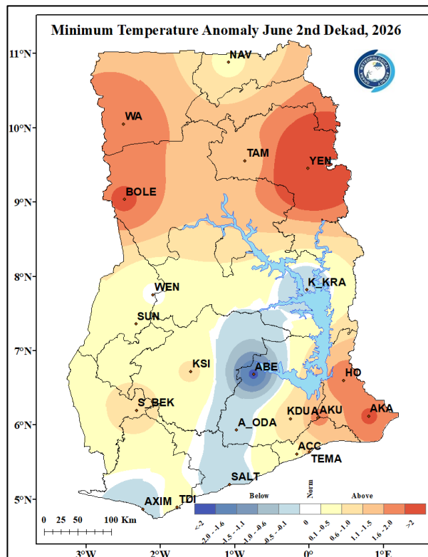
Figure 6b. Min. Temperature Anomaly June 2nd Dekad, 2026
