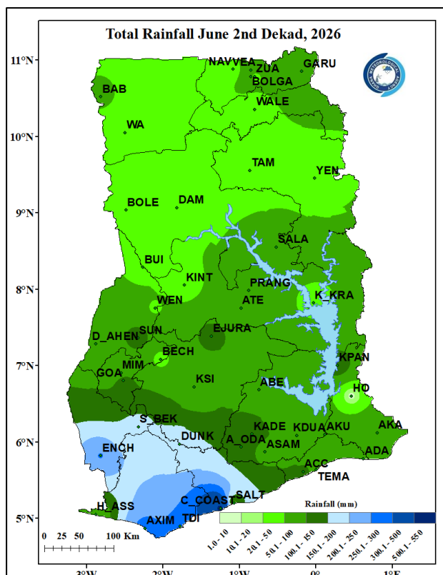
Figure 3a. Total Rainfall June 2nd Dekad, 2026
