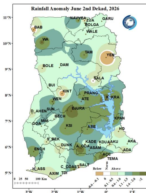
Figure 4 Rainfall Anomaly for June 2nd Dekad, 2026
