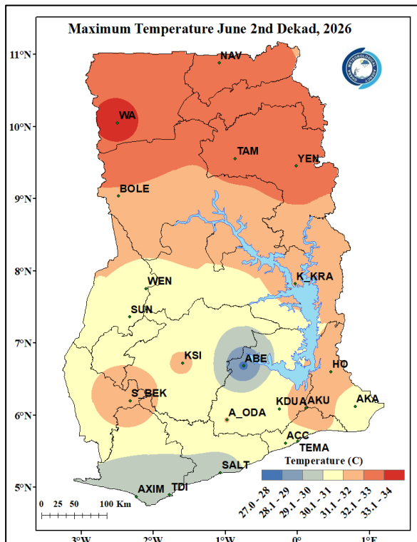
Figure 5a. Max Temperature June 2nd Dekad, 2026
