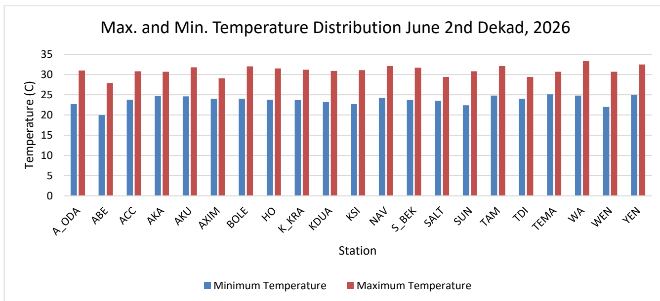
Figure 7 Max. and Min. Temperature Distribution for June 2nd Dekad, 2026
