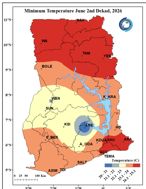
Figure 6 a. Min. Temperature June 2nd Dekad, 2026
