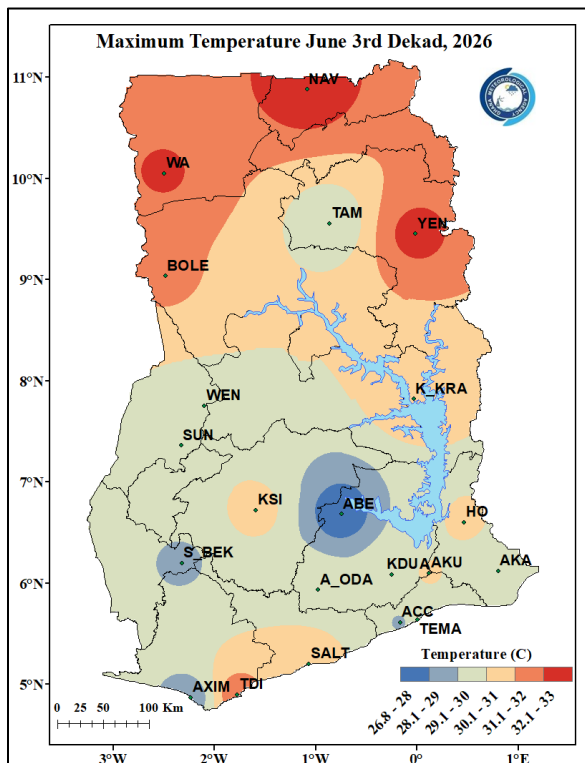
Figure 5a. Max Temperature June 3 rd Dekad, 2026
