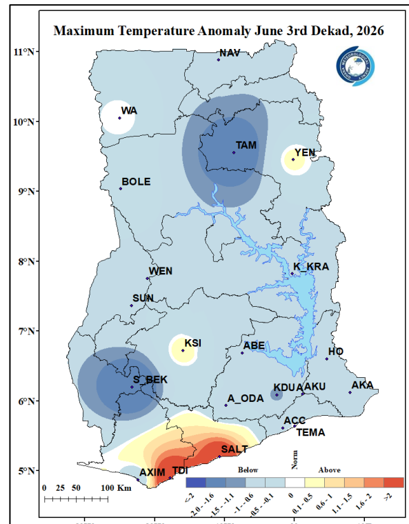
Figure 5b. Max. Temperature Anomaly June 3 rd Dekad, 2026
