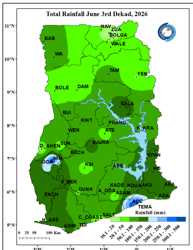
Figure 3a. Total Rainfall June 3 rd Dekad, 2026
