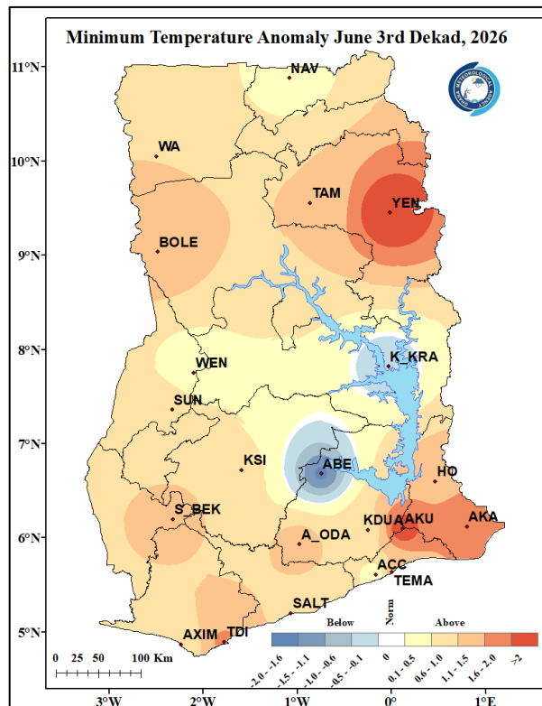
Figure 6b. Min. Temperature Anomaly June 3 rd Dekad, 2026
