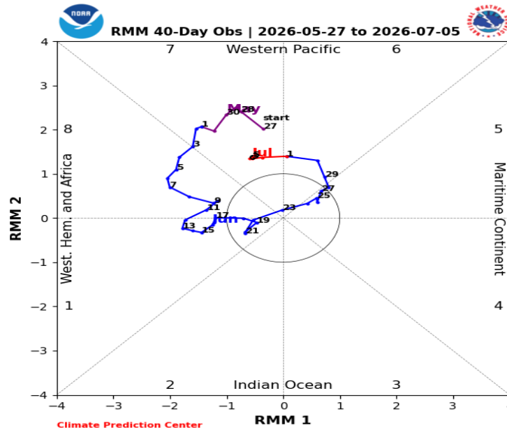
Figure 2. Current MJO position as of June 3 rd Dekad, 2026
