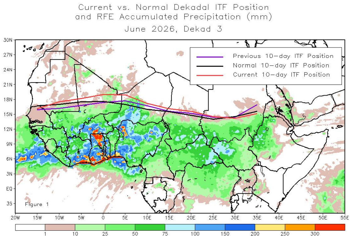
Figure 1. Current ITF position for June 3rd Dekad, 2026
