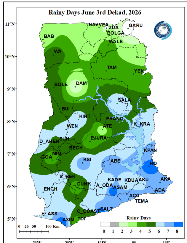
Figure 3b. Rainy Days June 3 rd Dekad, 2026
