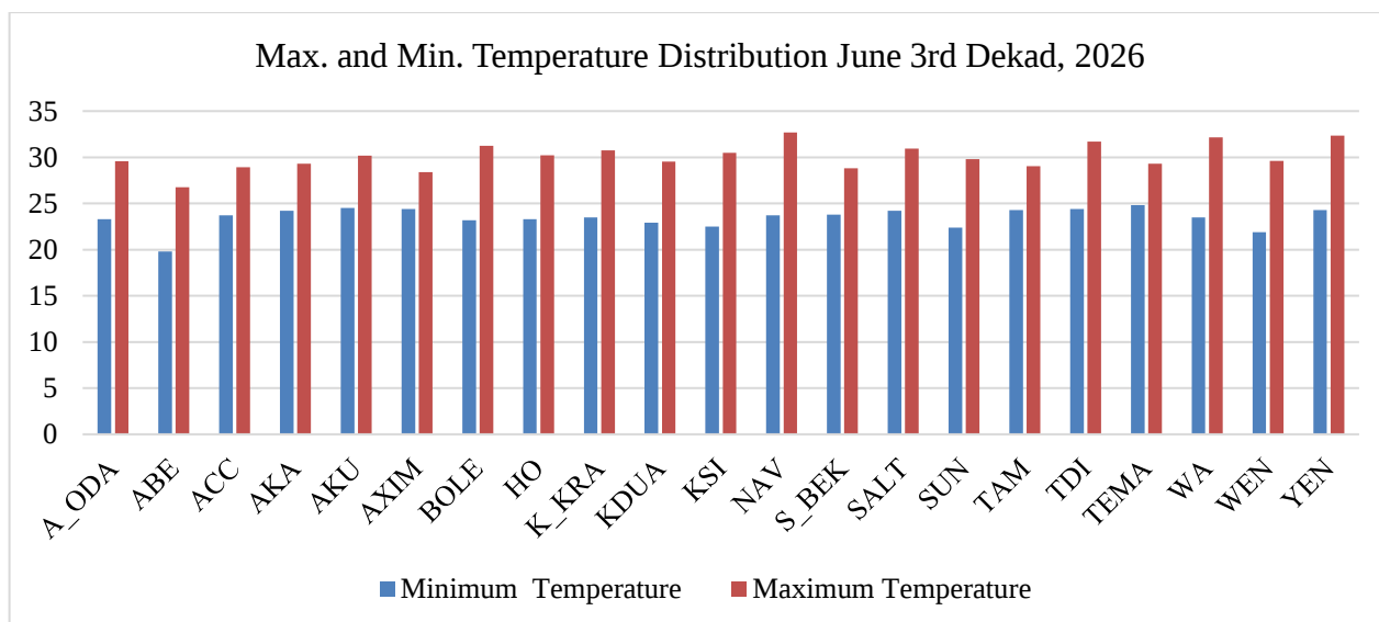
Figure 7 Max. and Min. Temperature Distribution for June 3 rd Dekad, 2026
