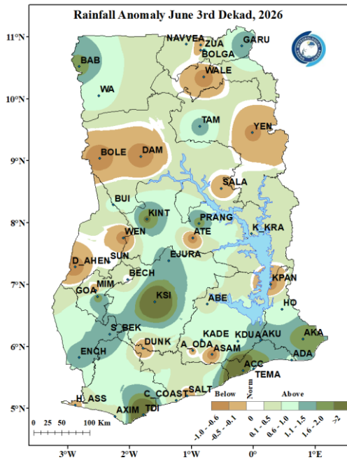
Figure 4 Rainfall Anomaly for June 3 rd Dekad, 2026
