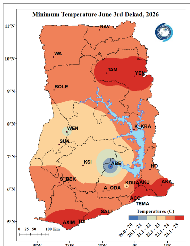
Figure 6 a. Min. Temperature June 3 rd Dekad, 2026
