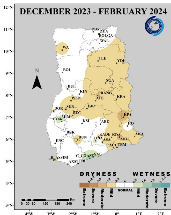
Fig. 1(b): 3-Month SPI (for agricultural drought): December 2023 – February 2024
