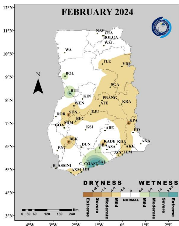
Fig. 1(a): 1-Month SPI (for meteorological drought): February 2024
