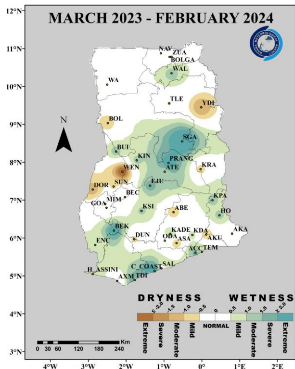
Fig. 1(d): 12-Month SPI (for streamflow and lake storage drought): March 2023 – February 2024
