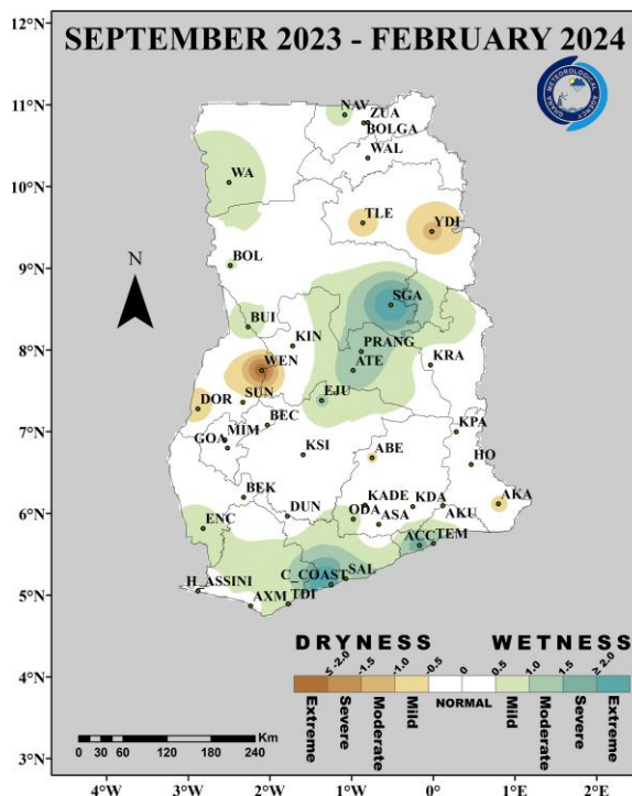
Fig. 1(c): 6-Month SPI (for hydrological drought): September 2023 – February 2024
