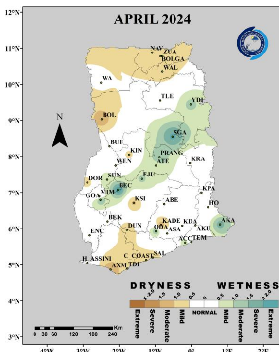
Fig. 1(a): 1-Month SPI (for meteorological drought): April 2024
