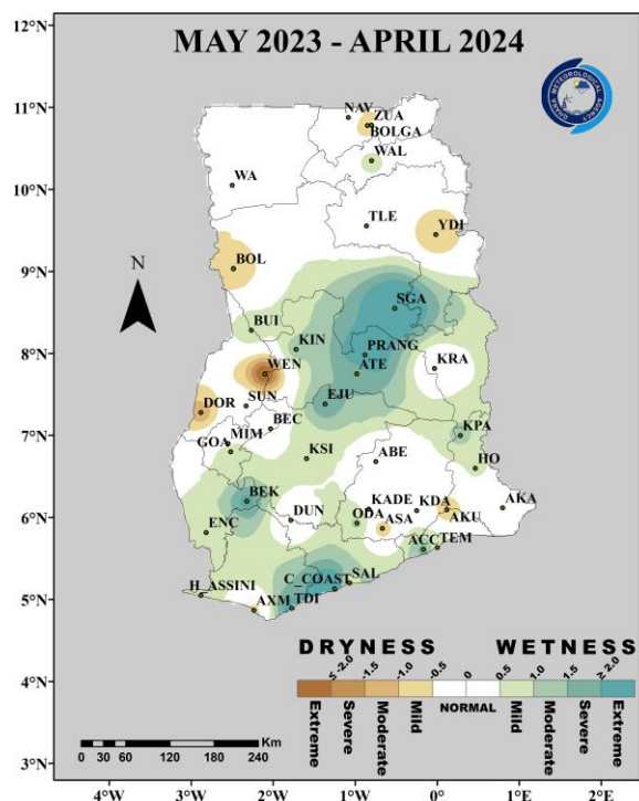
Fig. 1(d): 12-Month SPI (for streamflow and lake storage drought): May 2023 – April 2024
