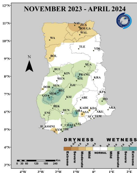
Fig. 1(c): 6-Month SPI (for hydrological drought): November 2023 – April 2024
