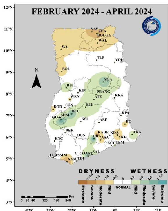
Fig. 1(b): 3-Month SPI (for agricultural drought): February 2024 – April 2024
