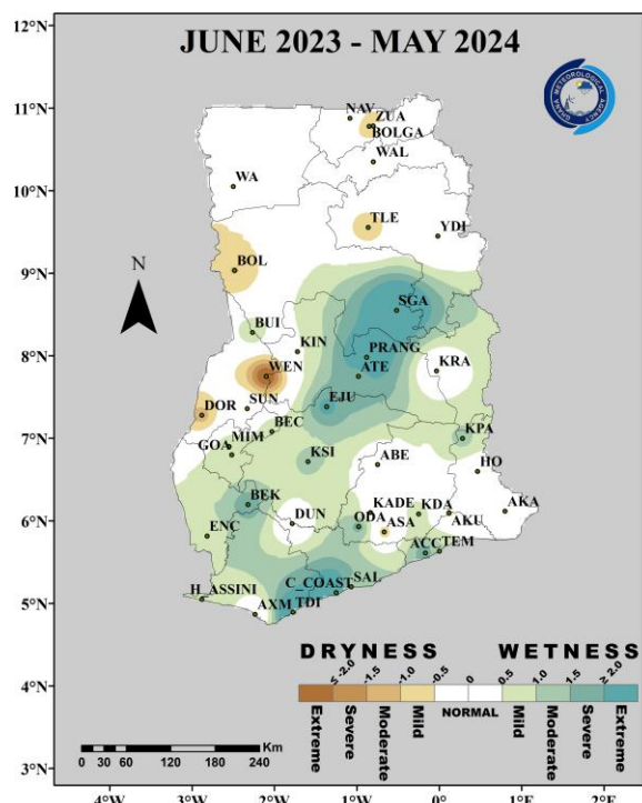
Fig. 1(d): 12-Month SPI (for streamflow and lake storage drought): June 2023 – May 2024
