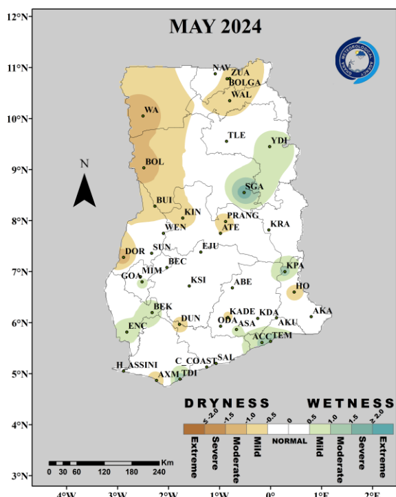
Fig. 1(a): 1-Month SPI (for meteorological drought): May 2024
