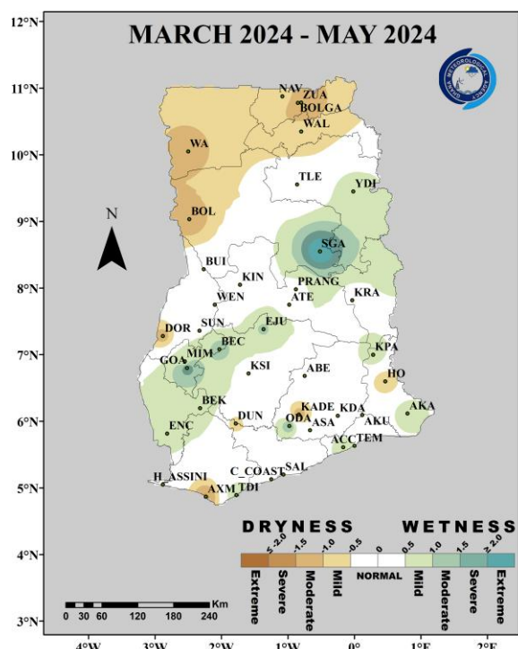
Fig. 1(b): 3-Month SPI (for agricultural drought): March 2024 – May 2024
