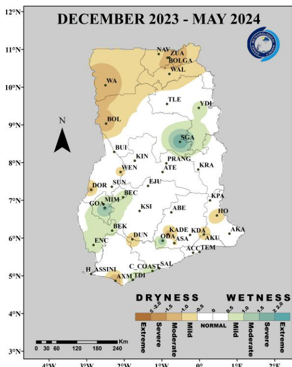
Fig. 1(c): 6-Month SPI (for hydrological drought): December 2023 – May 2024
