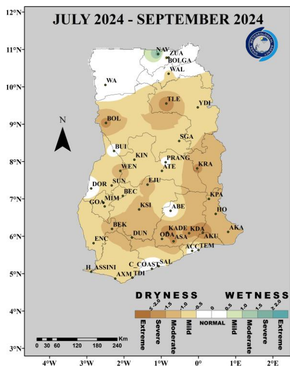
Fig. 1(b): 3-Month SPI (for agricultural drought): July 2024 – September 2024
