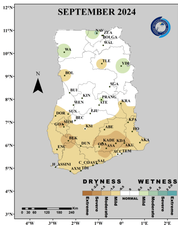
Fig. 1(a): 1-Month SPI (for meteorological drought): September 2024
