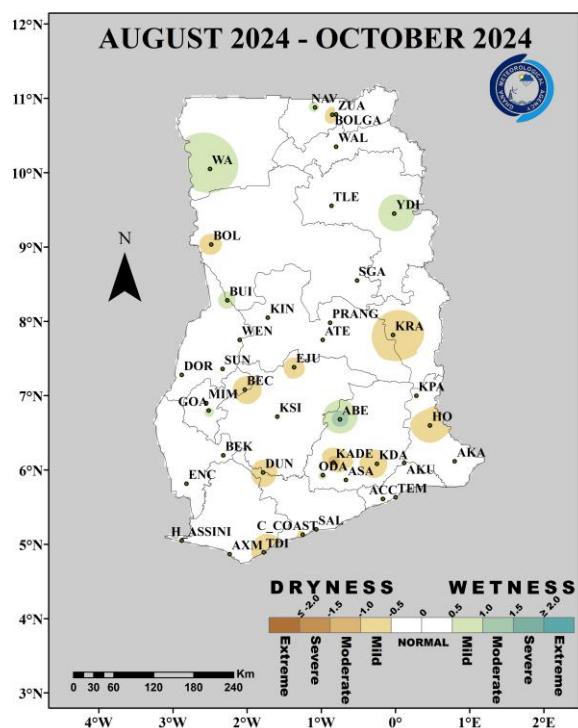
Fig. 1(b): 3-Month SPI (for agricultural drought): August 2024 – October 2024
