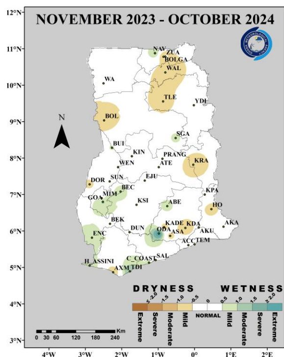
Fig 1(d): 12-Month SPI (for streamflow and lake storage drought): November 2023 – October 2024
