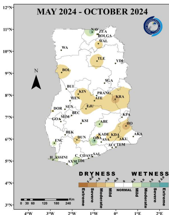
Fig 1(c): 6-Month SPI (for hydrological drought): May 2024 – October 2024
