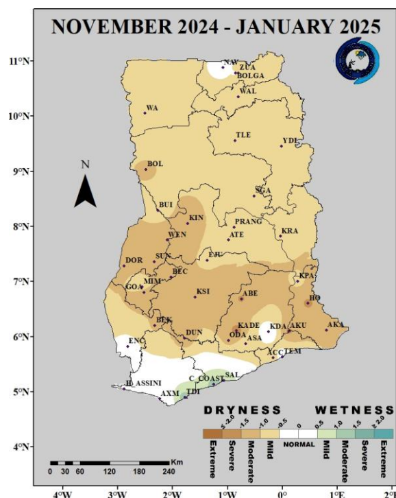
Fig. 1(b): 3-Month SPI (for agricultural drought): November 2024 – January 2025
