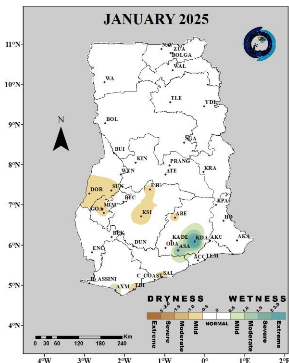
Fig. 1(a): 1-Month SPI (for meteorological drought): January 2025
