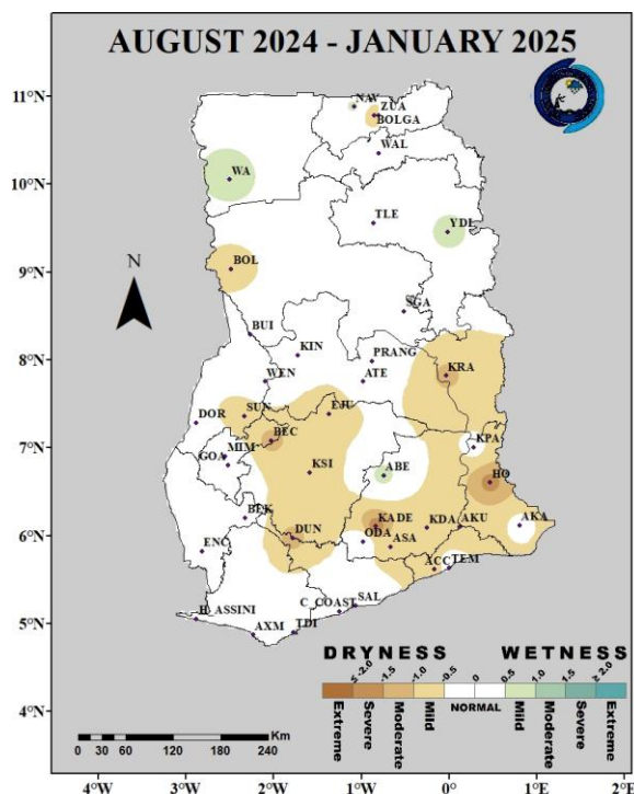
Fig. 1(c): 6-Month SPI (for hydrological drought): August 2024 – January 2025
