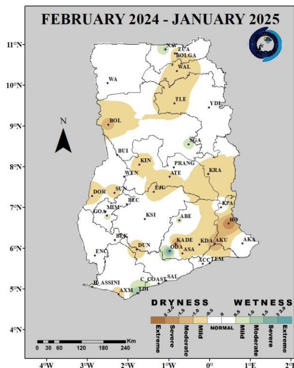
Fig. 1(d): 12-Month SPI (for streamflow and lake storage drought): February 2024 – January 2025
