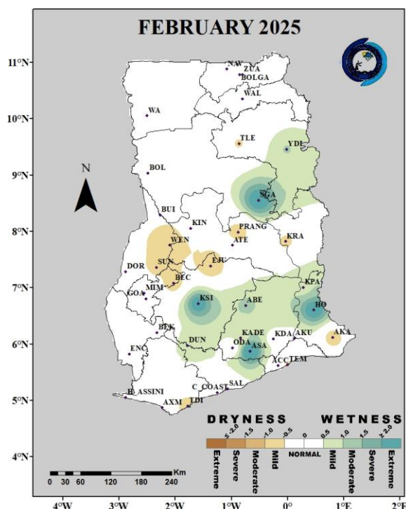
Fig. 1(a): 1-Month SPI (for meteorological drought): February 2025
