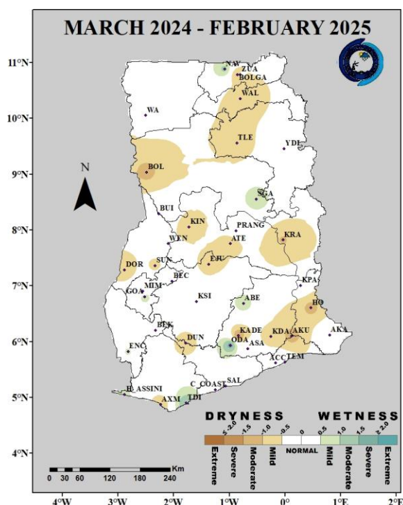
Fig. 1(d): 12-Month SPI (for streamflow and lake storage drought): March 2024 – February 2025
