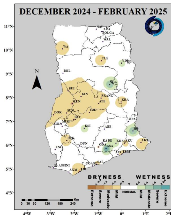
Fig. 1(b): 3-Month SPI (for agricultural drought): December 2024 – February 2025
