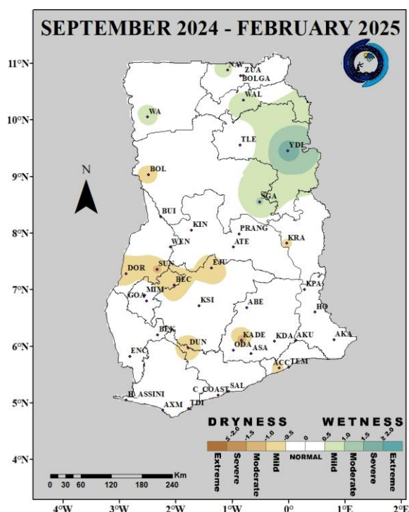
Fig. 1(c): 6-Month SPI (for hydrological drought): September 2024 – February 2025
