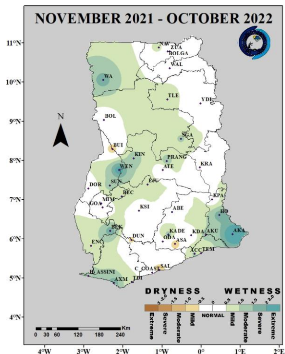
Fig 1(d): 12-Month SPI (for streamflow and lake storage drought): November 2021 – October 2022
