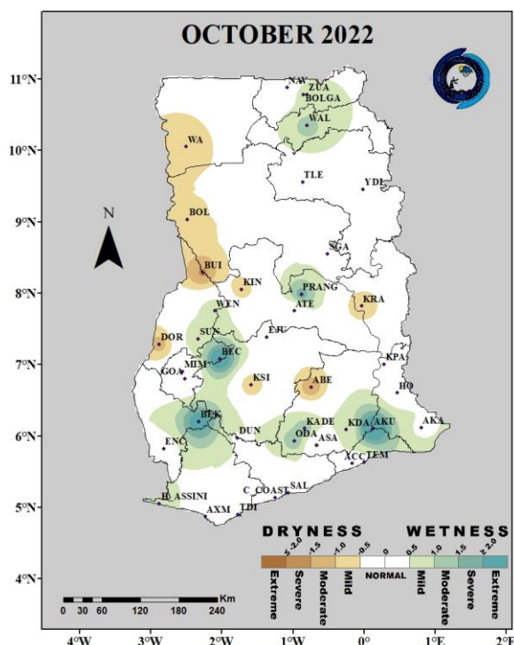
Fig. 1(a): 1-Month SPI (for meteorological drought): October 2022
