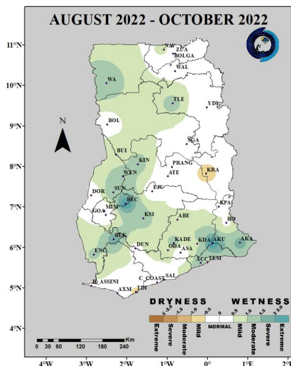
Fig. 1(b): 3-Month SPI (for agricultural drought): August 2022 – October 2022
