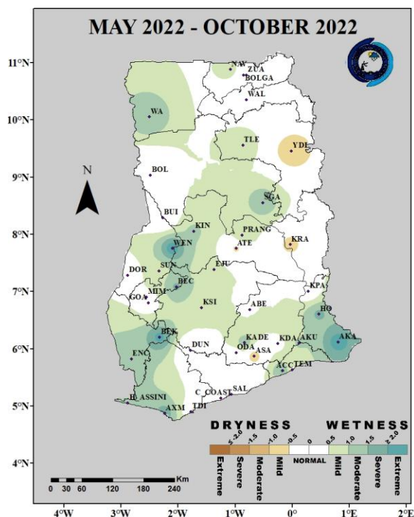
Fig. 1(c): 6-Month SPI (for hydrological drought): May 2022 – October 2022
