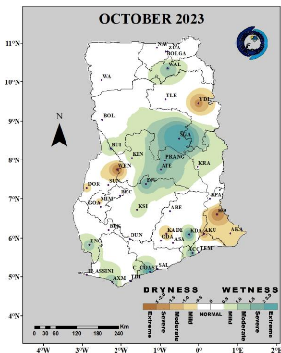
Fig. 1(a): 1-Month SPI (for meteorological drought): October 2023
