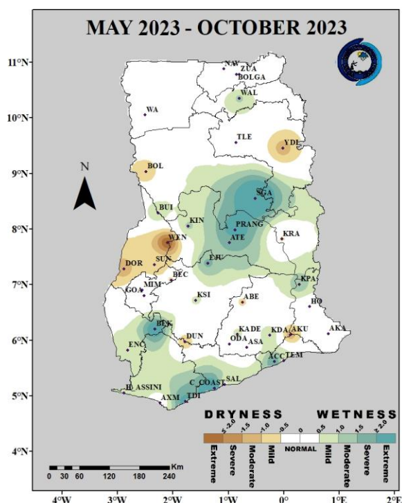
Fig 1(c): 6-Month SPI (for hydrological drought): May 2023 – October 2023
