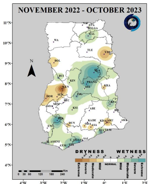
Fig 1(d): 12-Month SPI (for streamflow and lake storage drought): November 2022 – October 2023
