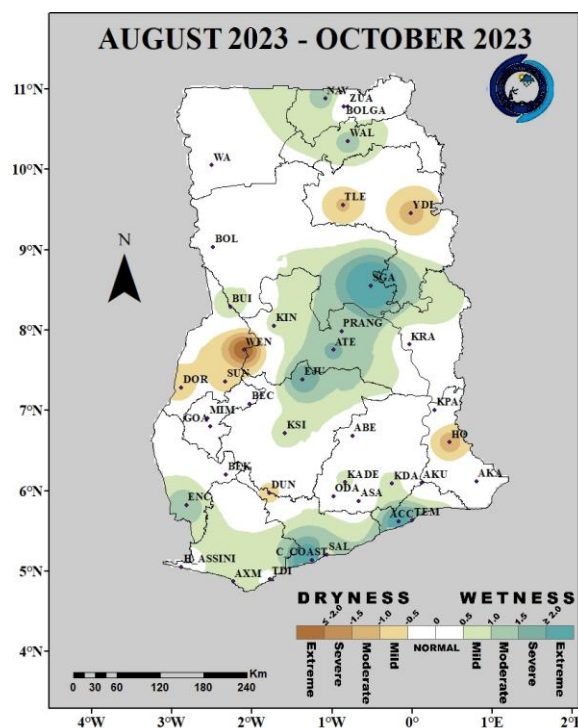
Fig. 1(b): 3-Month SPI (for agricultural drought): August 2023 – October 2023
