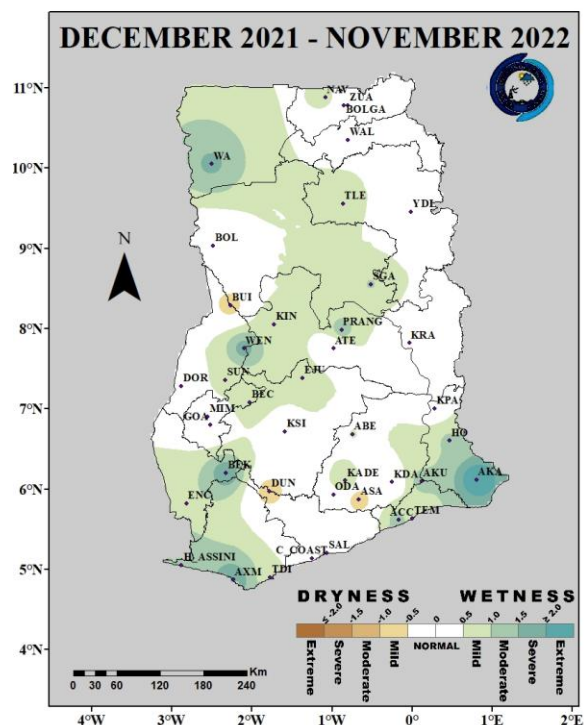
Fig. 1(d): 12-Month SPI (for streamflow and lake storage drought): December 2021 – November 2022
