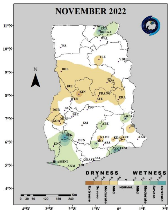
Fig. 1(a): 1-Month SPI (for meteorological drought): November 2022
