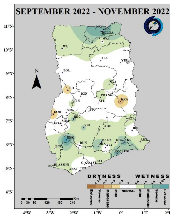
Fig. 1(b): 3-Month SPI (for agricultural drought): September 2022 – November 2022
