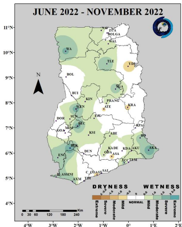
Fig. 1(c): 6-Month SPI (for hydrological drought): June 2022 – November 2022
