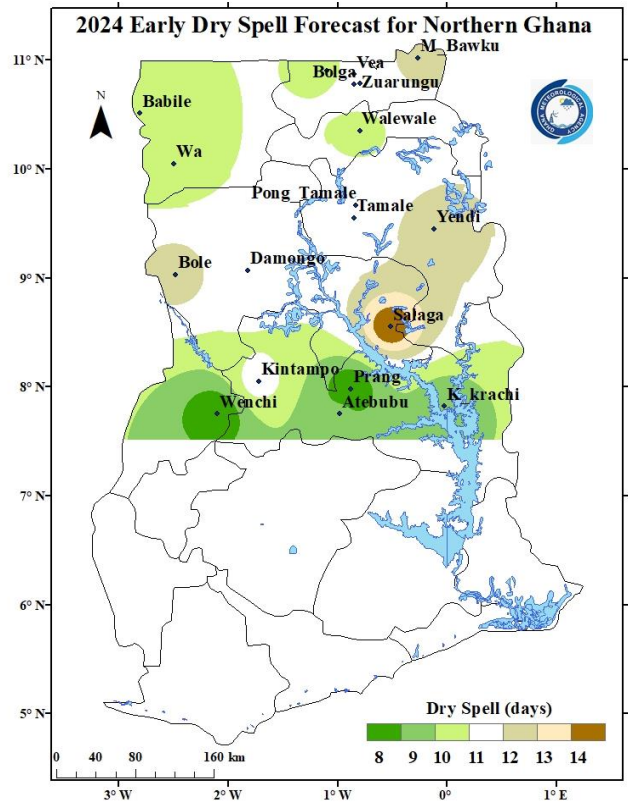
Fig.10 Early (1 st ) Dry Spell Forecast Map, 2024
