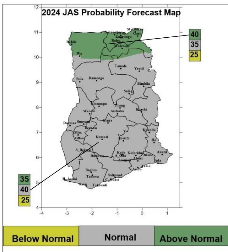
Fig.7 JAS Rainfall Probability Map, 2024
