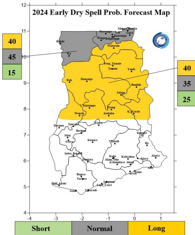
Fig.9 Early (1 st ) Dry Spell Probability Map, 2024
