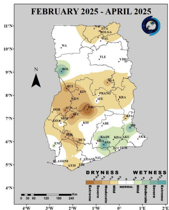
Fig. 1(b): 3-Month SPI (for agricultural drought): February 2025 – April 2025
