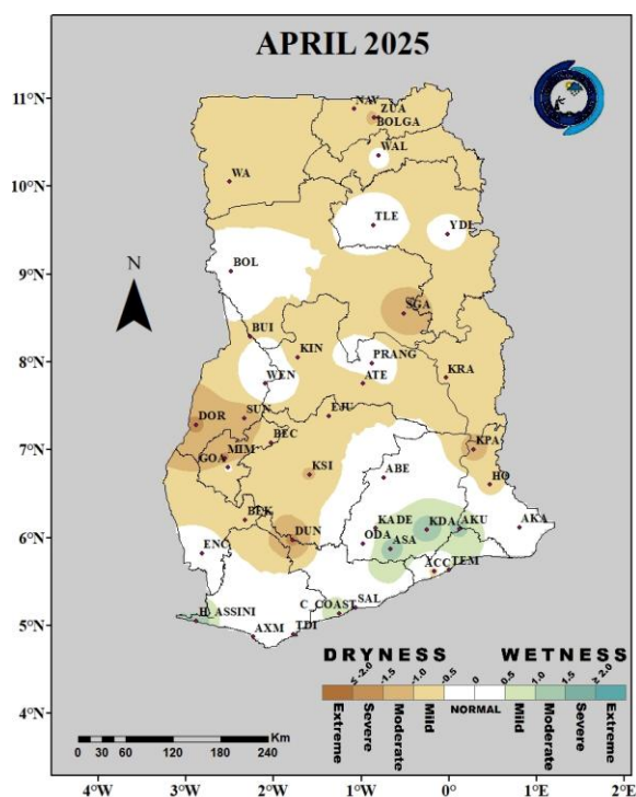
Fig. 1(a): 1-Month SPI (for meteorological drought): April 2025
