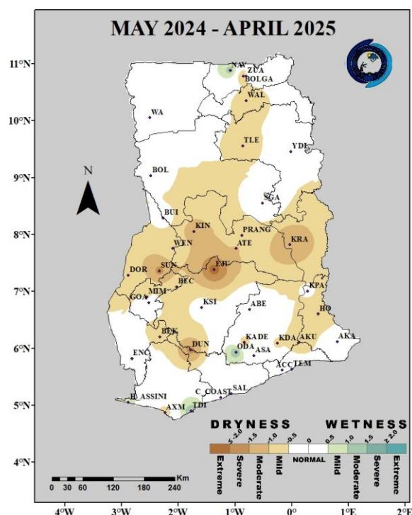
Fig. 1(d): 12-Month SPI (for streamflow and lake storage drought): May 2024 – April 2025
