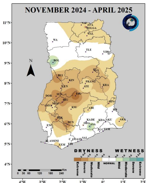
Fig. 1(c): 6-Month SPI (for hydrological drought): November 2024 – April 2025
