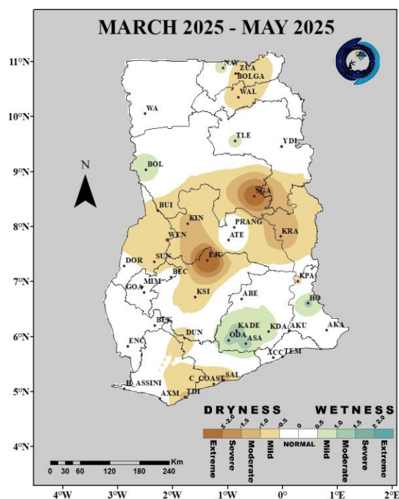
Fig. 1(b): 3-Month SPI (for agricultural drought): March 2025 – May 2025
