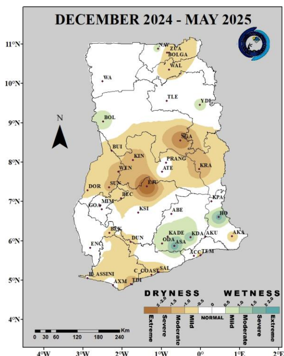
Fig. 1(c): 6-Month SPI (for hydrological drought): December 2024 – May 2025
