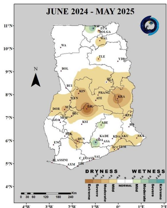
Fig. 1(d): 12-Month SPI (for streamflow and lake storage drought): June 2024 – May 2025
