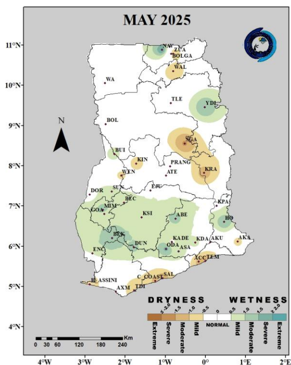
Fig. 1(a): 1-Month SPI (for meteorological drought): May 2025
