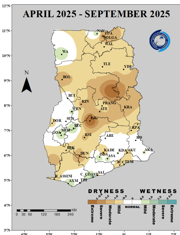
Fig. 1(c): 6-Month SPI (for hydrological drought): April 2025 – September 2025
