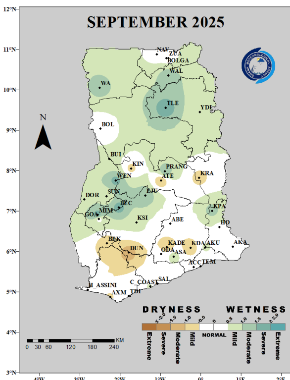
Fig. 1(a): 1-Month SPI (for meteorological drought): September 2025
