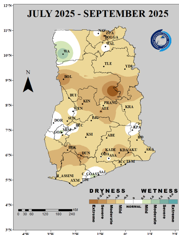
Fig. 1(b): 3-Month SPI (for agricultural drought): July 2025 – September 2025
