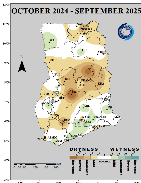
Fig. 1(d): 12-Month SPI (for streamflow and lake storage drought): October 2024 – September 2025
