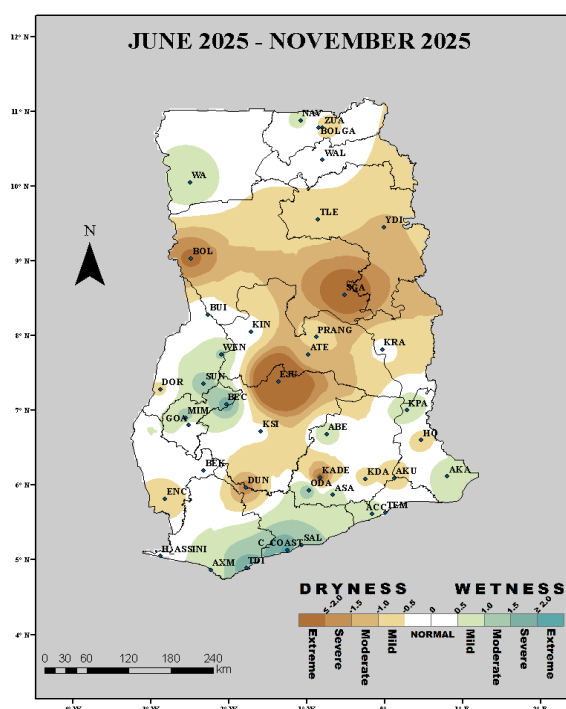
Fig. 1(c): 6-Month SPI (for hydrological drought): June 2025 – November 2025
