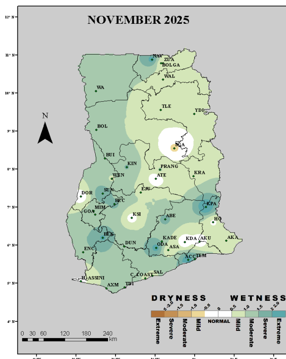
Fig. 1(a): 1-Month SPI (for meteorological drought): November 2025
