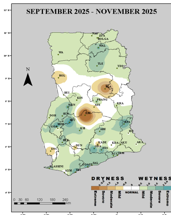
Fig. 1(b): 3-Month SPI (for agricultural drought): September 2025 – November 2025
