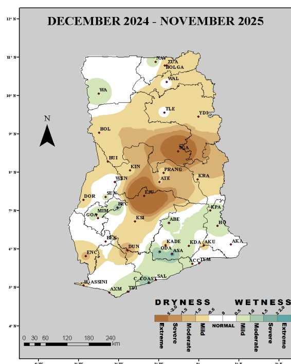
Fig. 1(d): 12-Month SPI (for streamflow and lake storage drought): December 2024 – November 2025
