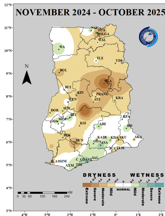
Fig. 1(d): 12-Month SPI (for streamflow and lake storage drought): November 2024 – October 2025
