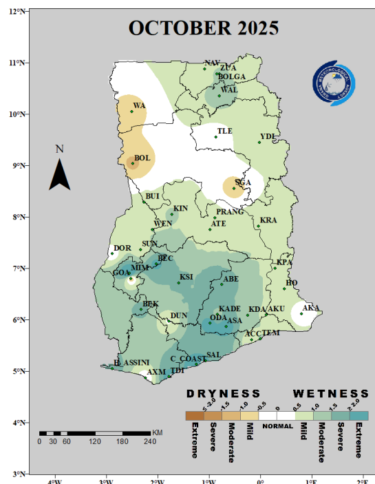
Fig. 1(a): 1-Month SPI (for meteorological drought): October 2025
