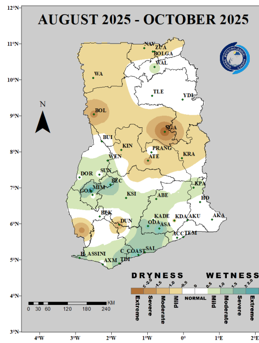
Fig. 1(b): 3-Month SPI (for agricultural drought): August 2025 – October 2025
