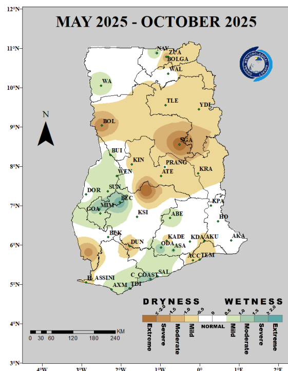
Fig. 1(c): 6-Month SPI (for hydrological drought): May 2025 – October 2025
